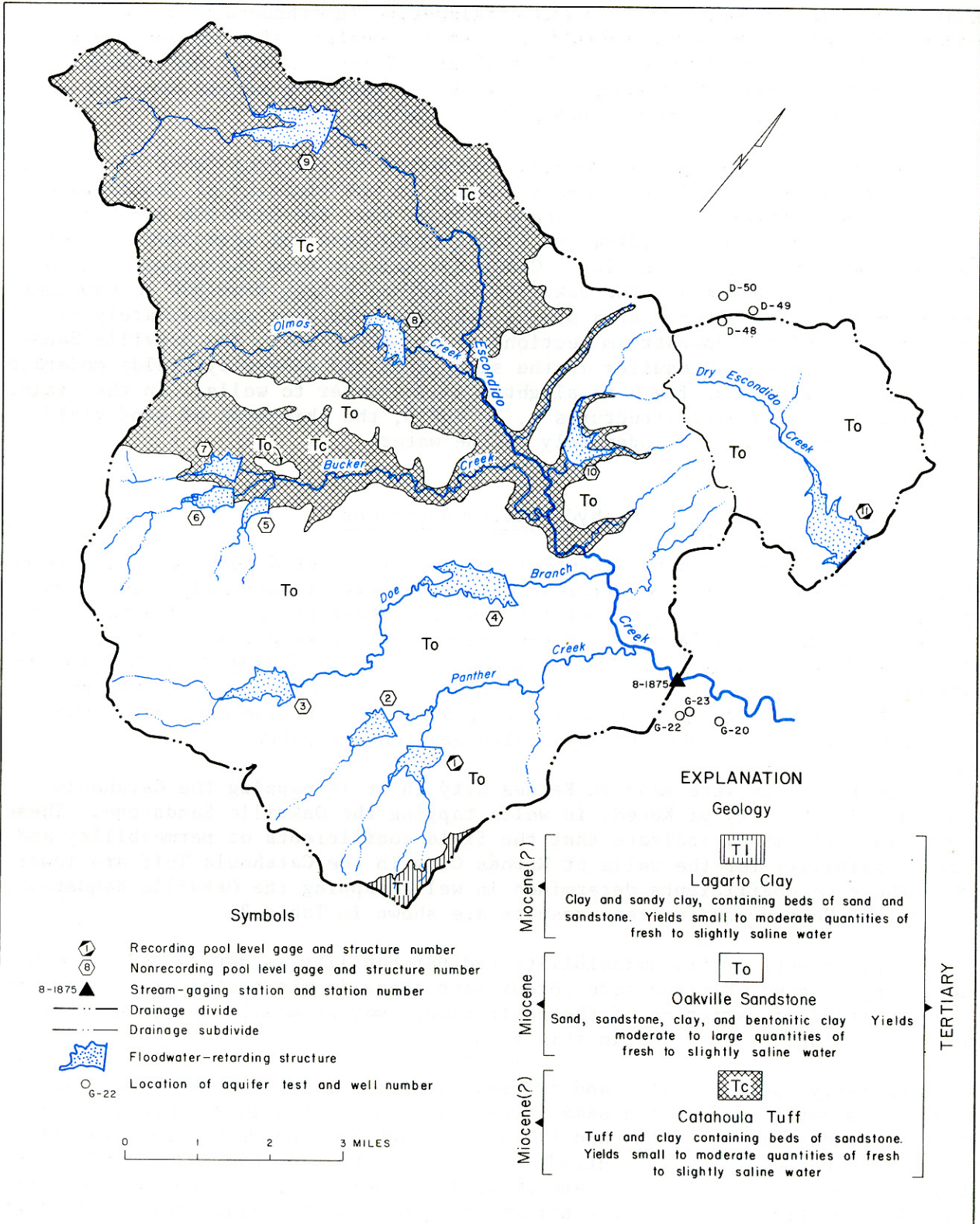
Figure 4 Geology of Study Area and Location of Test Wells and Floodwater - Retarding Structures
